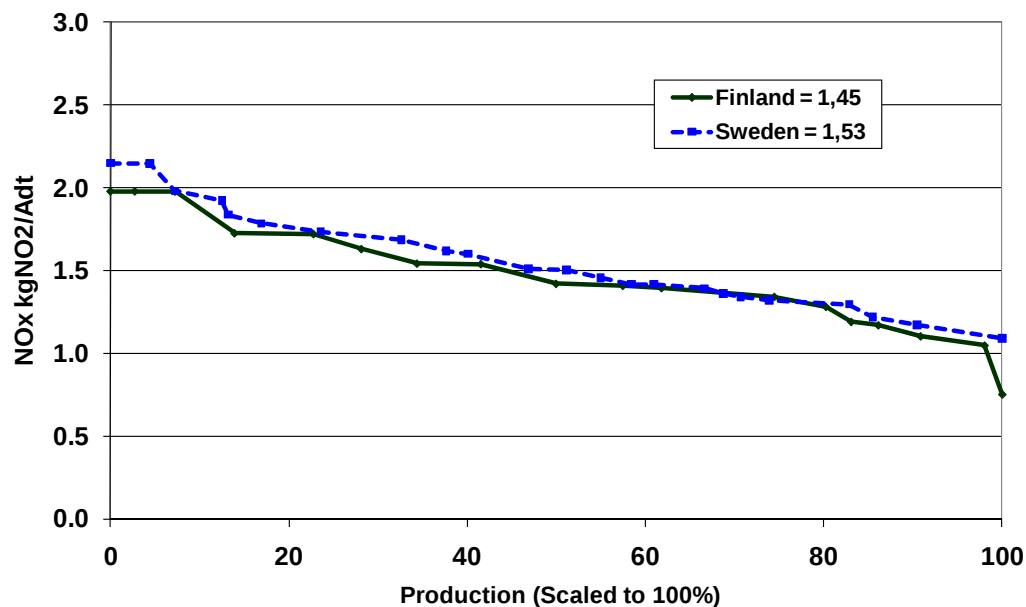
Figure 1: Average yearly emissions from Swedish and Finnish recovery boilers from year 2003.
