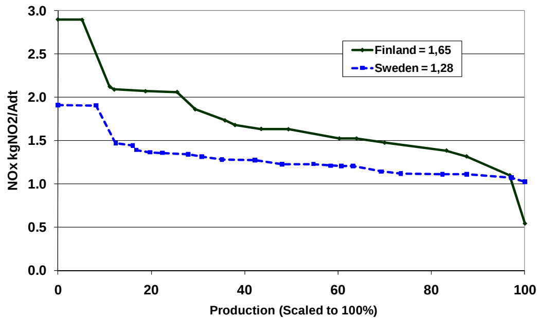
Figure 2: Average yearly emissions from Swedish and Finnish recovery boilers from year 2008.
