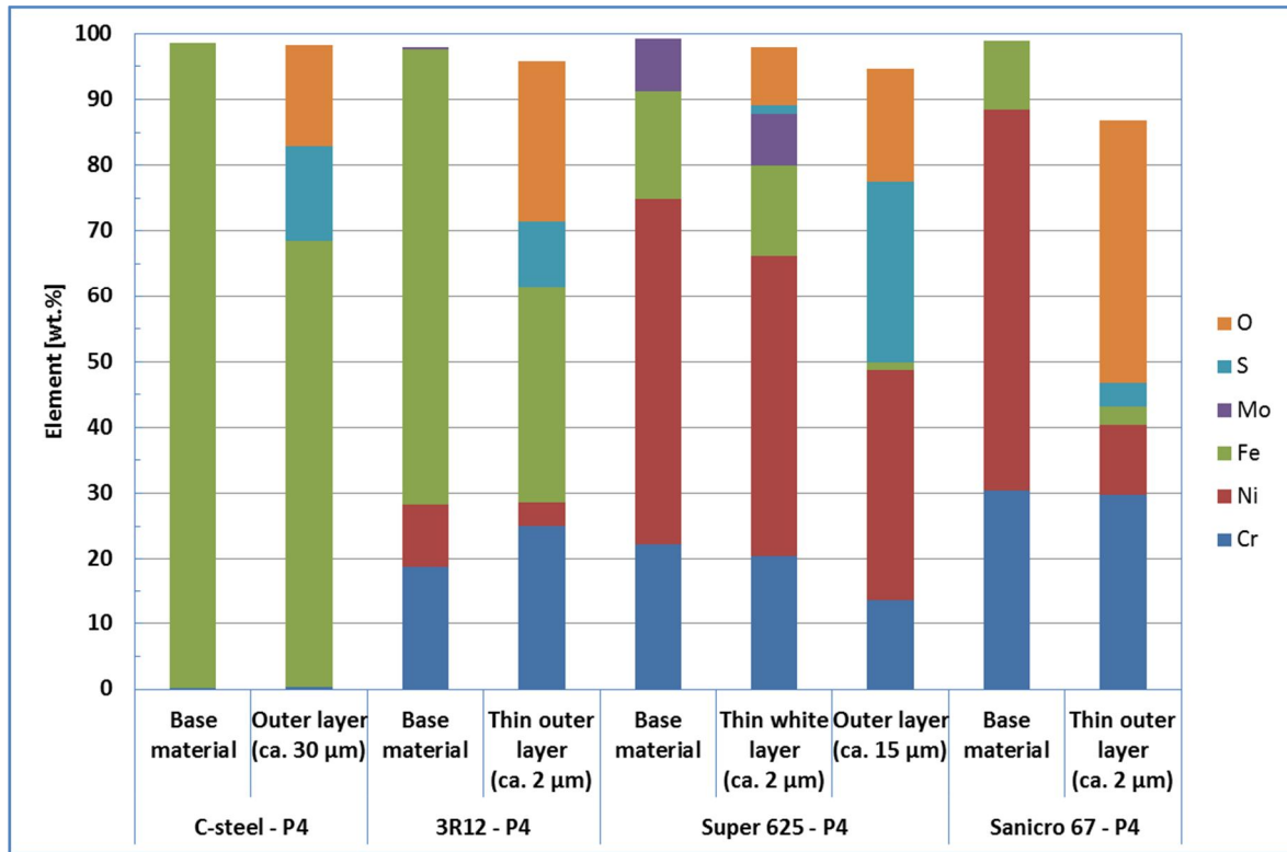
Figure 50. Results from the EDS analysis performed for the carbon steel, 3R12, Sanicro 67 and Super 625 after 2154 h exposure in lower furnace at 440 °C (Probe test No. 4). Note: Quantitative results from cross sections, carbon excluded. Data from layers are from point analysis, whereas area analysis was used for base materials.
