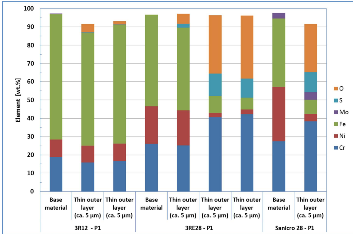
Figure 14. Results from the EDS analysis performed for the 3R12, 3RE28 and Sanicro 28 specimens after 906 h exposure in lower furnace at 440 °C (Probe test No. 1). Note: Quantitative results from cross sections, carbon excluded. Data from layers are from point analysis, whereas area analysis was used for base materials.
