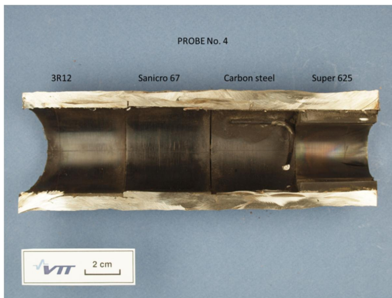
Figure 39. Macrographs taken from the probe No. 4 head after exposure: a) outer surface exposed to the furnace side and b) inner surface exposed to the cooling liquid. A thermocouple soldered on the side surface of carbon steel specimen is clearly visible on inner surface.
