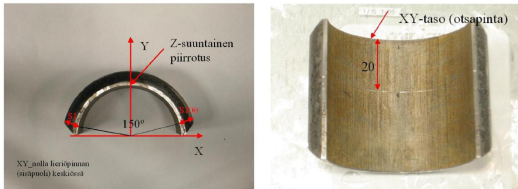
Figure 1. The wall thickness profiles were measured before and after testing with coordinate measurement machine a) as a function of circumference b) from three axial locations ( Z = 15, 25 and 32 mm).
