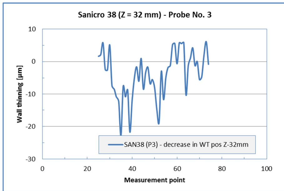
Figure 33. Circumferential wall thinning curves from Sanicro 38 specimen (Probe No. 3): a) axial location Z = 25 mm and b) axial location Z = 32 mm.
