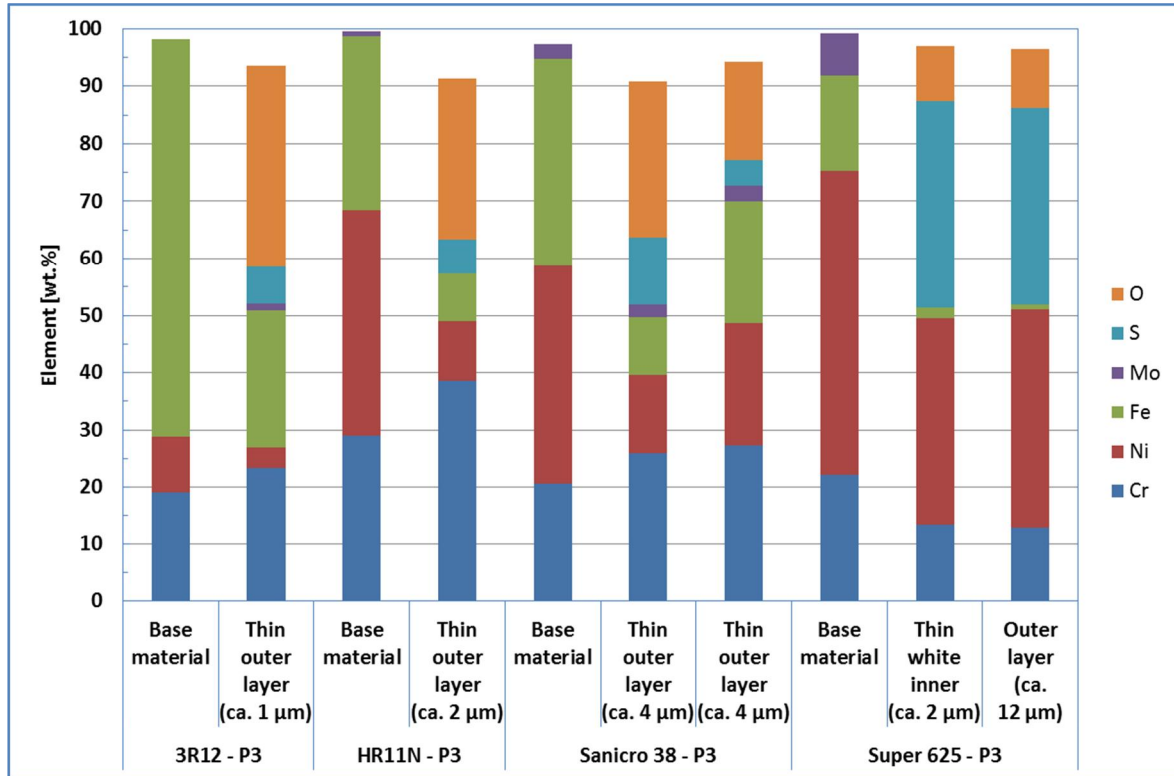
Figure 38. Results from the EDS analysis performed for the 3R12, HR11N, Sanicro 38 and Super 625 specimens after 750 h exposure in lower furnace at 430 °C (Probe test No. 3). Note: Quantitative results from cross sections, carbon excluded. Data from layers are from point analysis, whereas area analysis was used for base materials.
