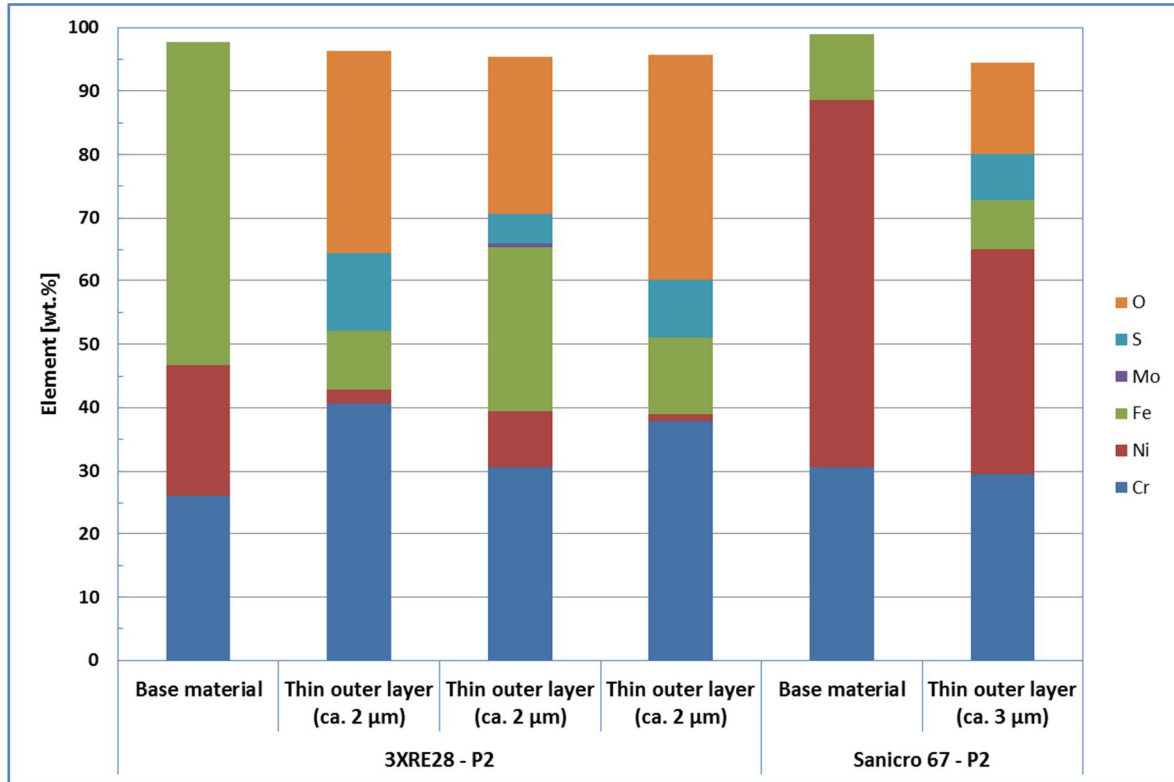
Figure 26. Results from the EDS analysis performed for the 3XRE28 and Sanicro 67 specimens after 744 h exposure in lower furnace at 440 °C (Probe test No. 2). Note: Quantitative results from cross sections, carbon excluded. Data from layers are from point analysis, whereas area analysis was used for base materials.
