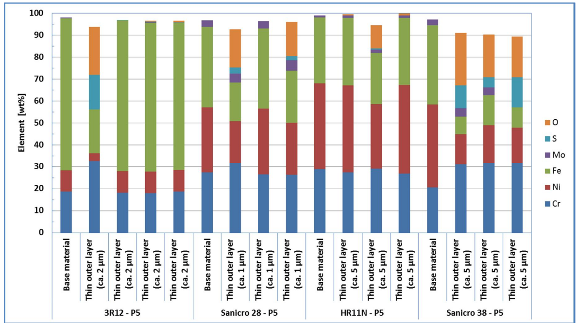
Figure 60. Results from the EDS analysis performed for the 3R12, Sanicro 28, HR11N and Sanicro 38 after 2157 h exposure in lower furnace at 440 °C (Probe test No. 5). Note: Quantitative results from cross sections, carbon excluded. Data from layers are from point analysis, whereas area analysis was used for base materials.
