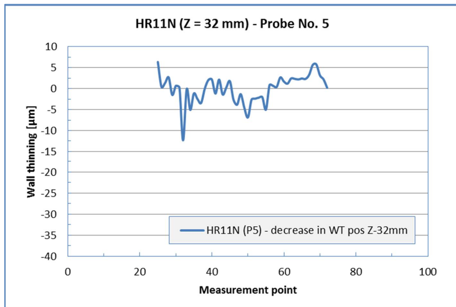
Figure 55. Circumferential wall thinning curves from HR11N specimen (Probe No. 5): a) axial location Z = 25 \text{ mm} and b) axial location Z = 32 \text{ mm} .
