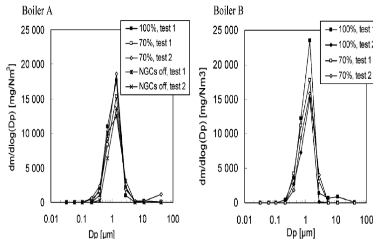
FIGURE 2. Particle mass size distributions at the ESP inlet at boilers A and B as determined with low-pressure impactors. The particles collected in the precutter cyclone (larger than 4\ \mu\text{m} ) are not included in the figures.
